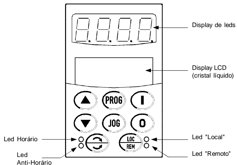
Figura 4.1 - HMI-SSW06
