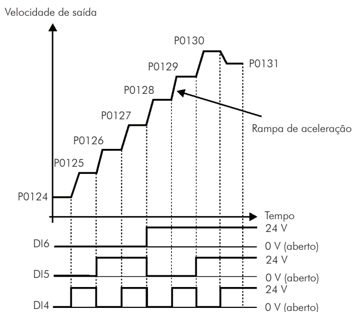
Figura 12.4 - Multispeed
