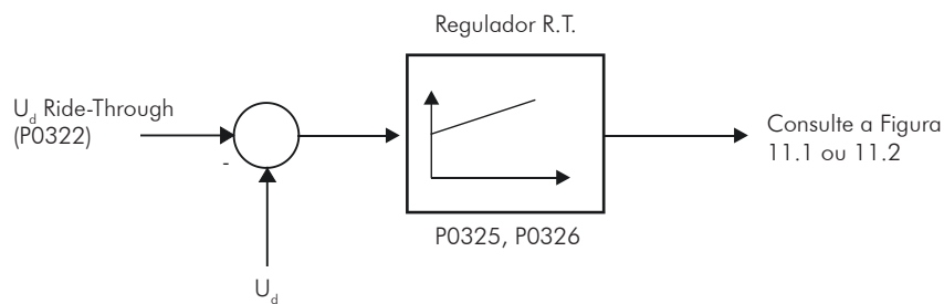
Figura 12.9 - Controlador PI do Ride-Through
